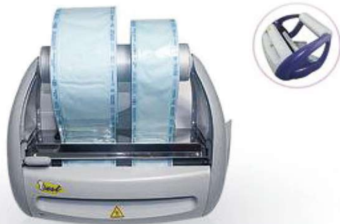
Order code MY-320 封口机 ☆ Voltage AC110v-240v ☆ Power 100w ☆ Seal width12mm ☆ Seal length 25cm ☆ Seal duration 3min ☆ Wall-mount/desktop
